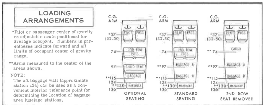
Figure 6-3. Loading Arrangements
