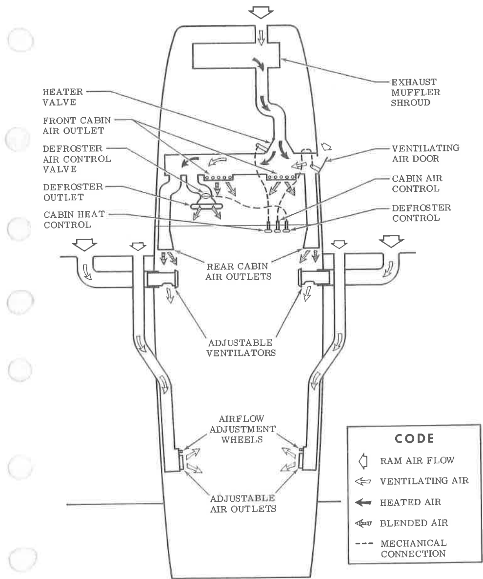
Figure 7-8. Cabin Heating, Ventilating, and Defrosting System
