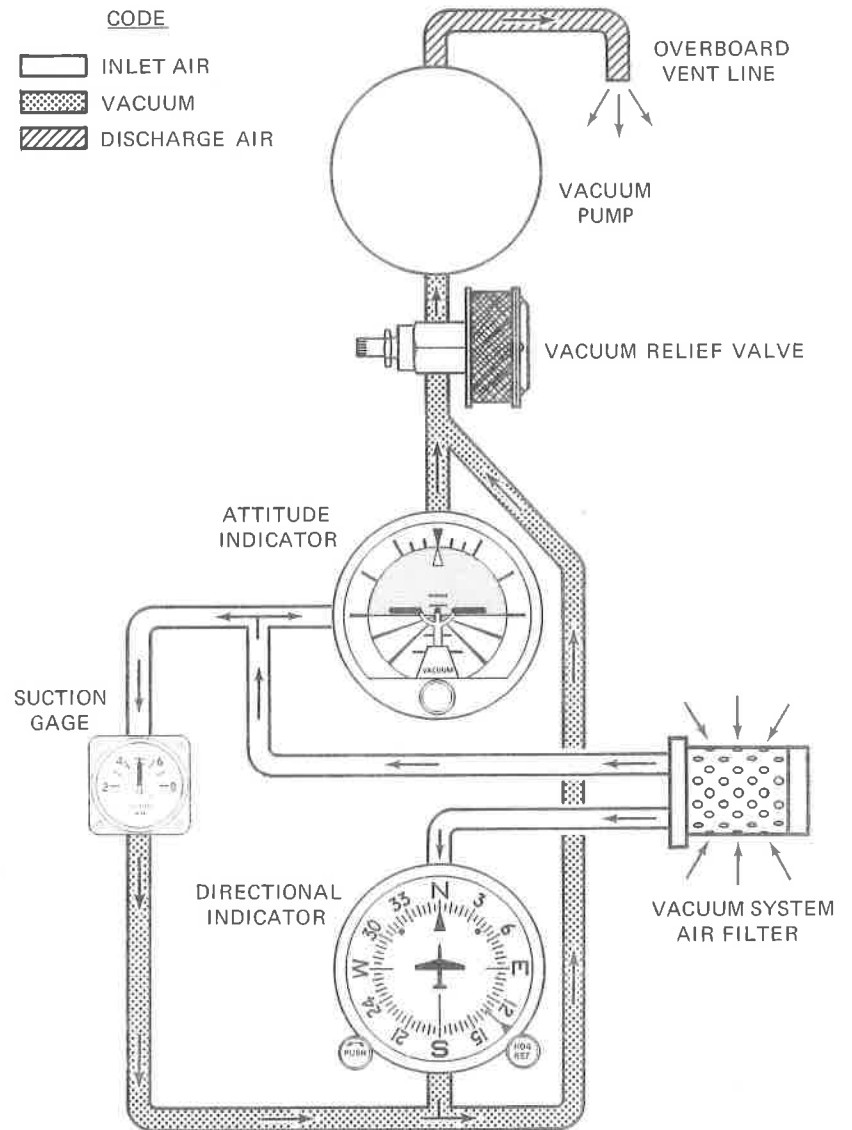
Figure 7-9. Vacuum System
