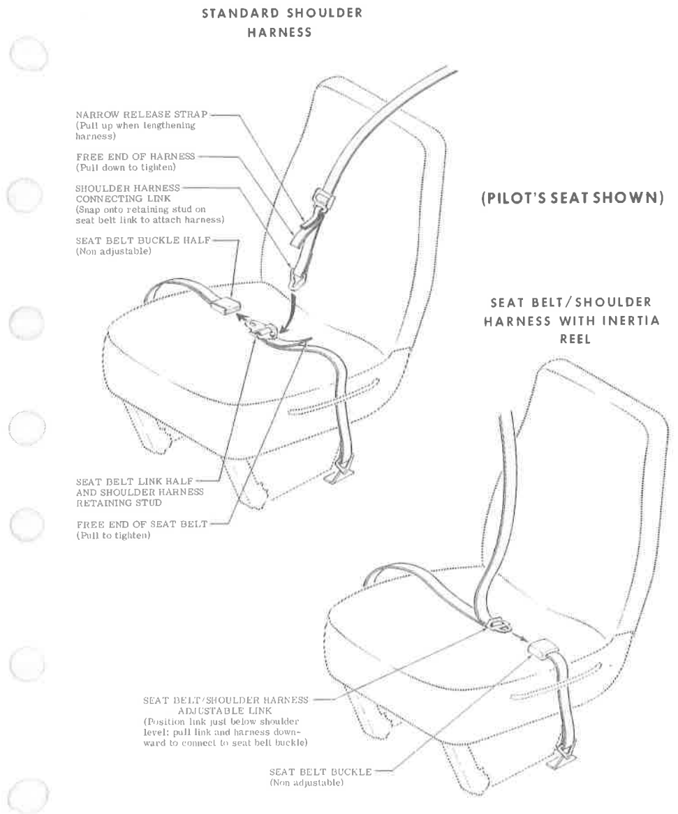
Figure 7-4. Seat Belts and Shoulder Harnesses
