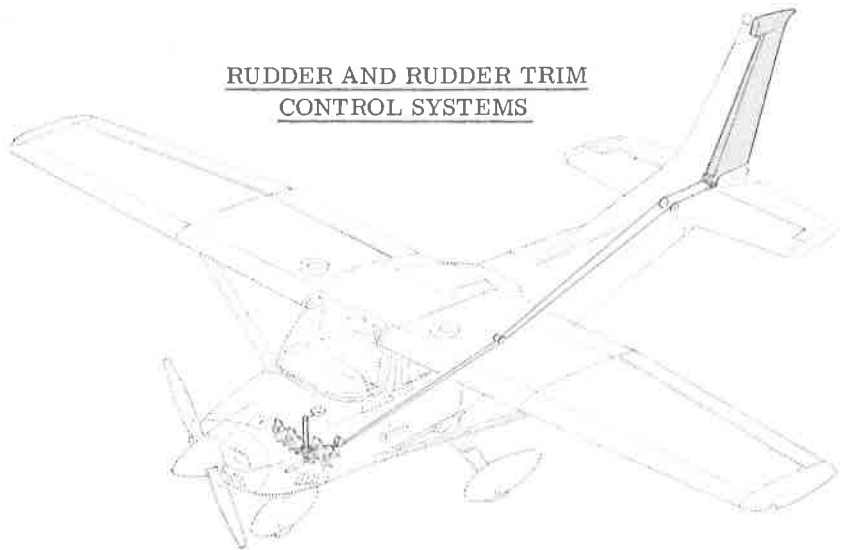
Figure 7-1. Flight Control and Trim Systems (Sheet 1 of 2)
