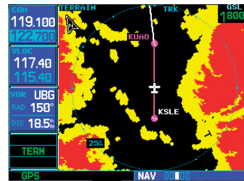
TERRAIN Page with 360° View
