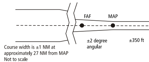
Full-Scale deflection and defined path for VTF approach
